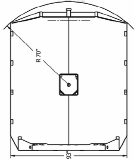
ALL STEEL AERODYNAMIC 9'4" FLAT GOOSE TOP VIEW 60" CA - DRW
