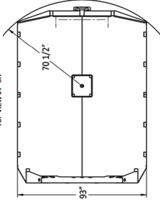
ALL STEEL AERODYNAMIC 11'4" FLAT GOOSE TOP VIEW 84" CA
